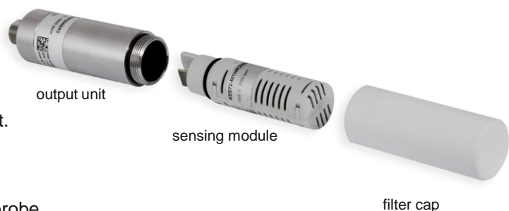
Fig. 5 EE872 modular construction
